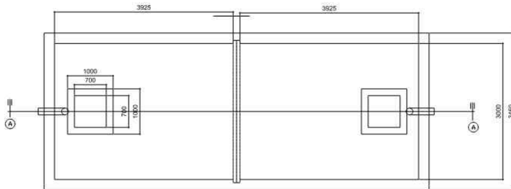
PLAN SCALE 1:40
